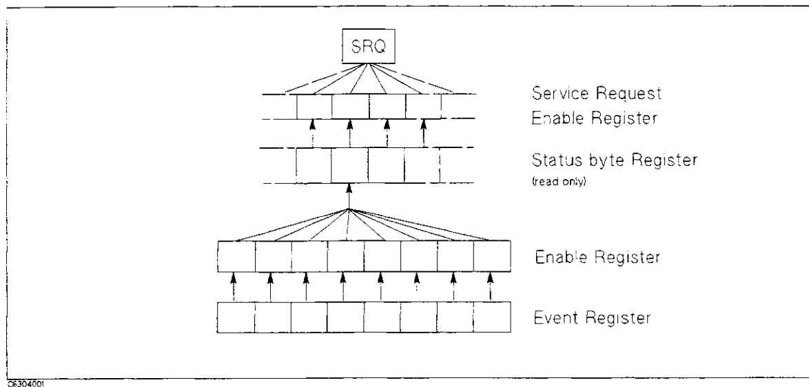
Figure 4-1. General Status Register Model
